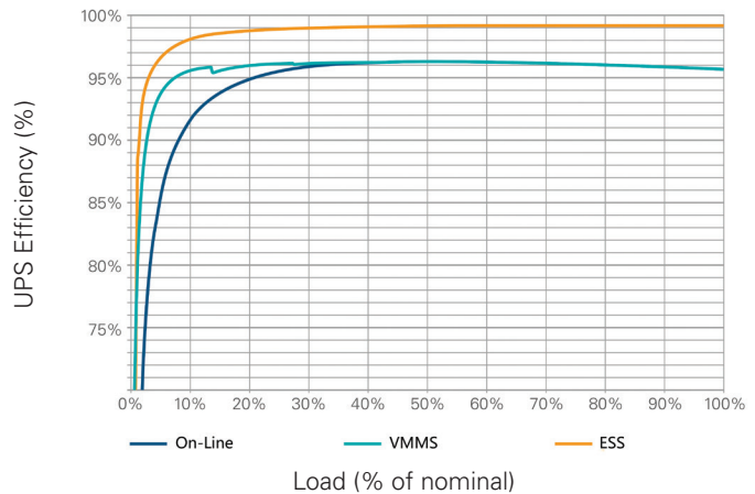
Eaton 93PR Efficiency in all modes
